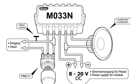
ANSCHLUSSPLAN | CONNECTING PLAN
